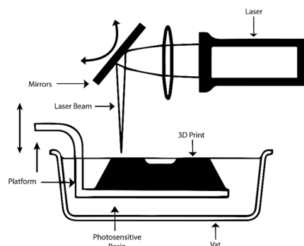
Figure 1. A basic schematic of stereolithography technology.
