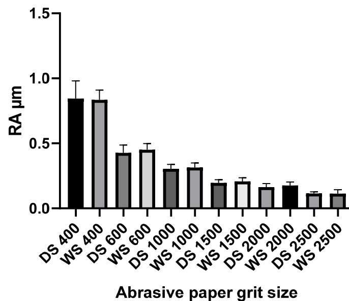
Figure 12. Fine sanding surface roughness comparison of wet vs. dry procedure on grouped orientations.
