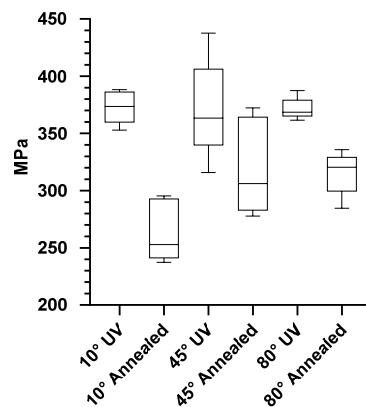
Figure 7. Flexural modulus results for UV vs. annealed groups of plaques in orientations of 10°, 45°, and 80°.
