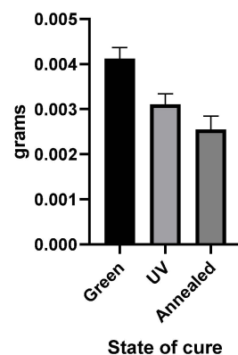
Figure 10. Weight loss results from abrasive blasting procedures in green, UV, and annealed states of cure.
