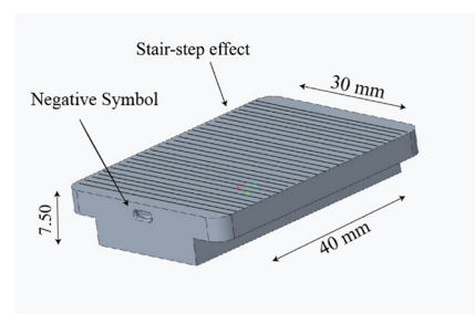
Figure 3. Dimensions of 3D-printed plaques (length 40.00 mm, width 30.00 mm, height 7.50 mm).
