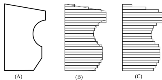
Figure 2. (A); Outline of CAD geometry, (B); outline of CAD geometry after slicing, (C); 3D-printed outline of layers.
