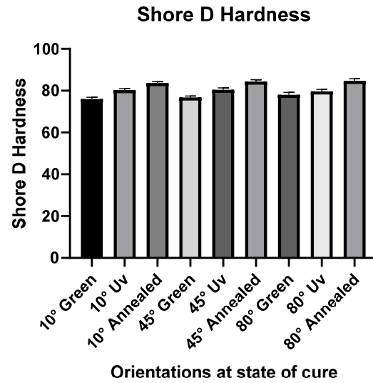
Figure 8. Overview of shore D hardness results on selected orientation of 10°, 45°, and 80° in green, UV-cured, and UV-cured and annealed state of cure.
