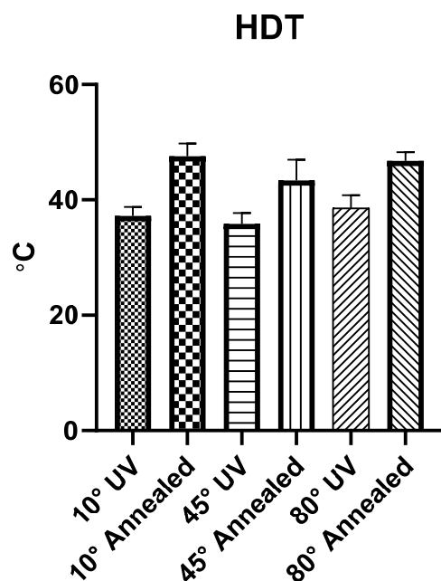
Figure 5. HDT comparison results from UV vs. annealed plaques fabricated in orientations of 10°, 45°, and 80°.
