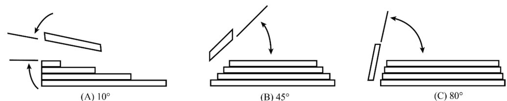
Figure 4. Illustration of the stair-step effect built at (A) 10°, (B) 45°, and (C) 80° orientations.
