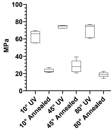
Figure 6. Flexural strength results for UV vs. annealed groups of plaques in orientations of 10°, 45°, and 80°.
