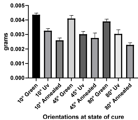
Figure 9. Overview of dry sanding weight removal results on plaques printed in orientations of 10°, 45°, and 80° at green, UV-cured, and annealed stages of cure.
