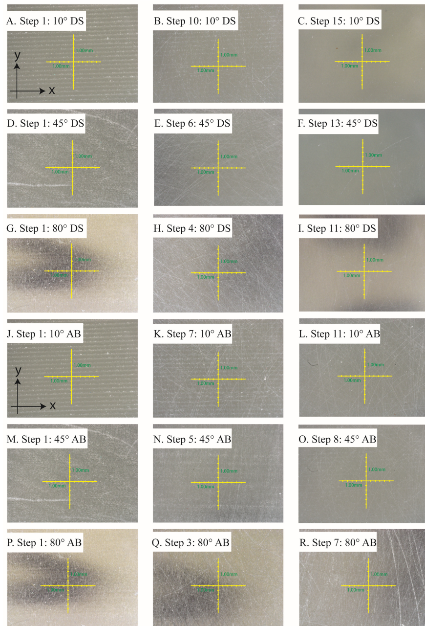
Figure 11. Microscopic images show removal of the stair-step effect on 10°, 45°, and 80° orientations at steps before, during, and after dry sanding (DS) in image; (A–I), and abrasive blasting (AB) in images (J–R).
